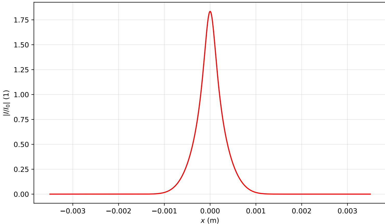
Intensity profile I(x, y = 0, z = 0.239)/I_0 , P_{in}=7.5P_{cr} , artificial time
